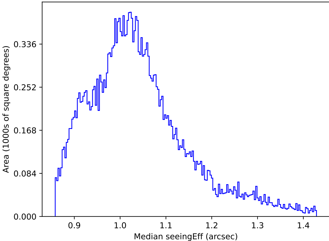
too_elab_r32_d2_griz_v3.4_10yrs All sky z band: Median seeingEff
