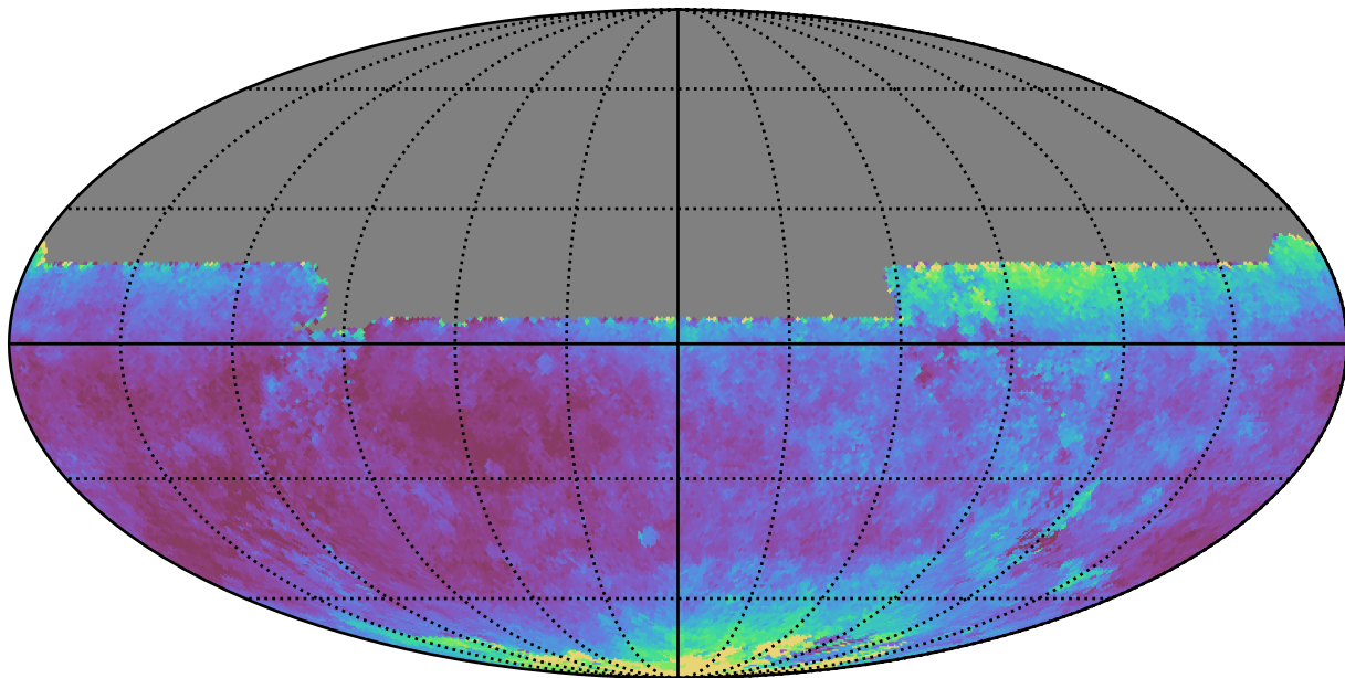
too_elab_r32_d2_griz_v3.4_10yrs All sky y band: Median seeingEff
