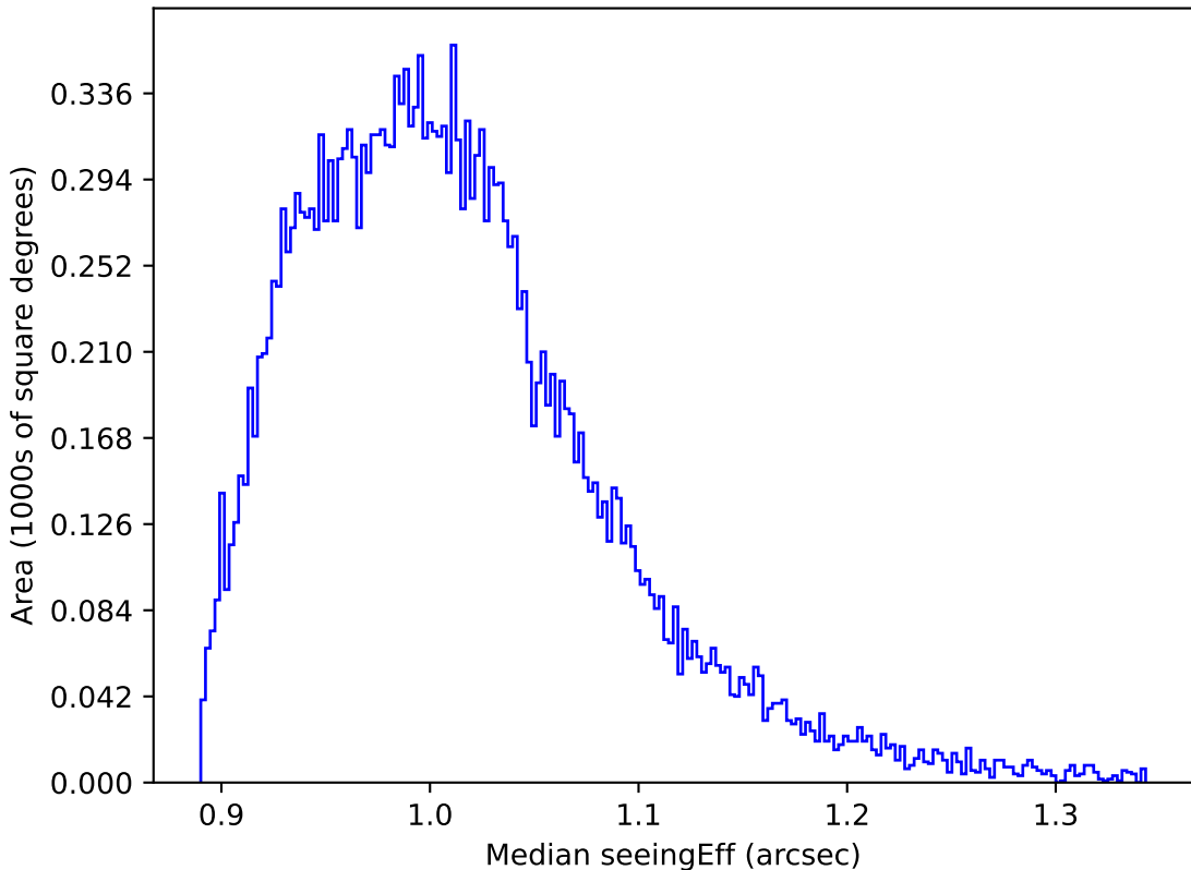
too_elab_r32_d2_griz_v3.4_10yrs All sky y band: Median seeingEff
