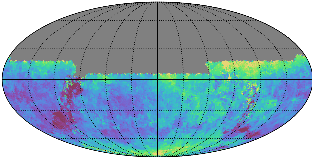
too_elab_r32_d2_griz_v3.4_10yrs All sky u band: Median seeingEff
