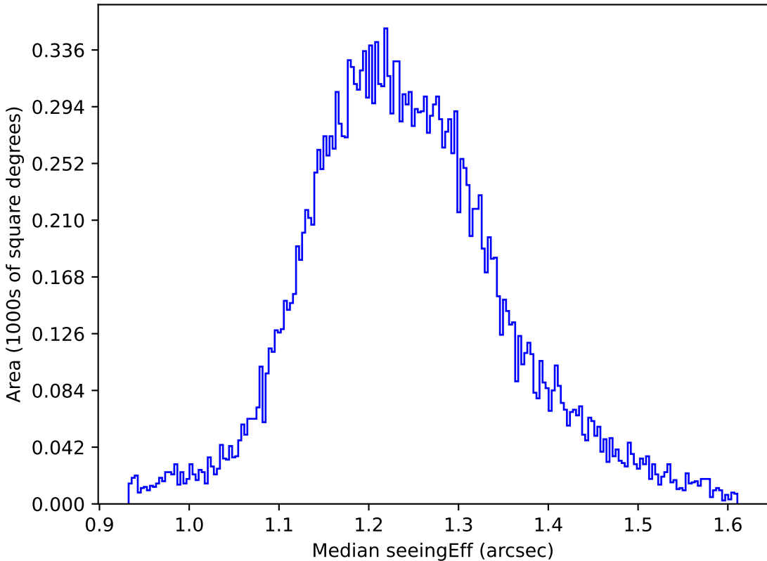
too_elab_r32_d2_griz_v3.4_10yrs All sky u band: Median seeingEff
