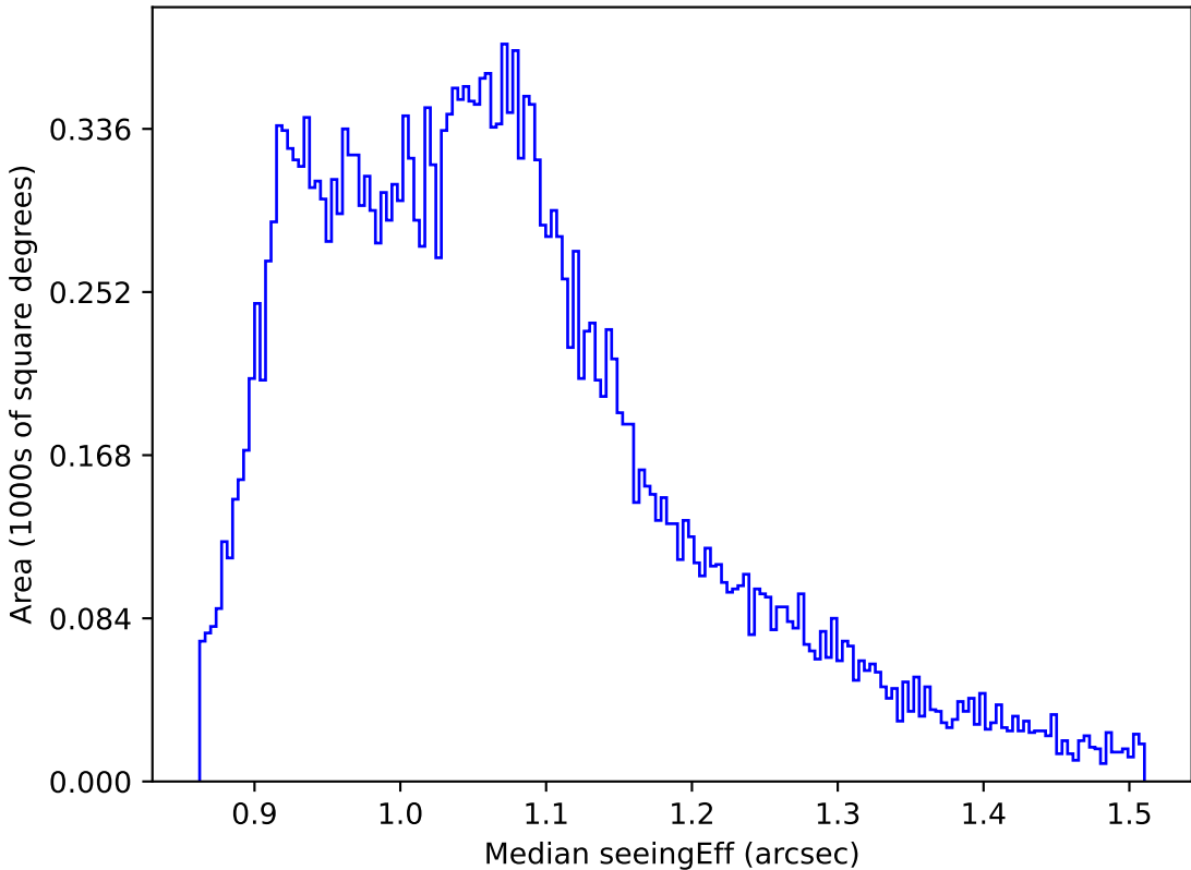
too_elab_r32_d2_griz_v3.4_10yrs All sky r band: Median seeingEff
