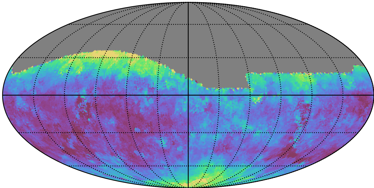
too_elab_r32_d2_griz_v3.4_10yrs All sky g band: Median seeingEff
