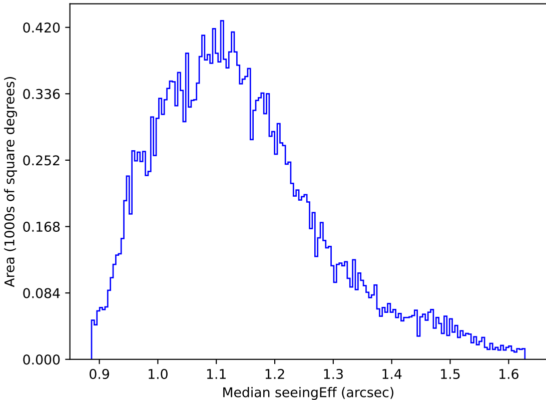
too_elab_r32_d2_griz_v3.4_10yrs All sky g band: Median seeingEff
