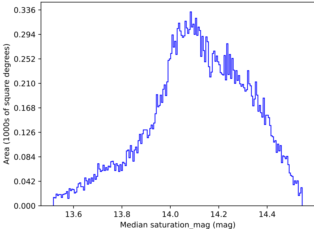
too_elab_r32_d2_griz_v3.4_10yrs All sky all bands: Median saturation_mag
