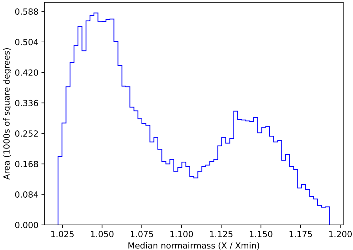
too_elab_r32_d2_griz_v3.4_10yrs WFD z band: Median normairmass
