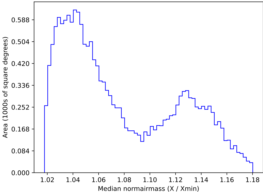
too_elab_r32_d2_griz_v3.4_10yrs WFD i band: Median normairmass
