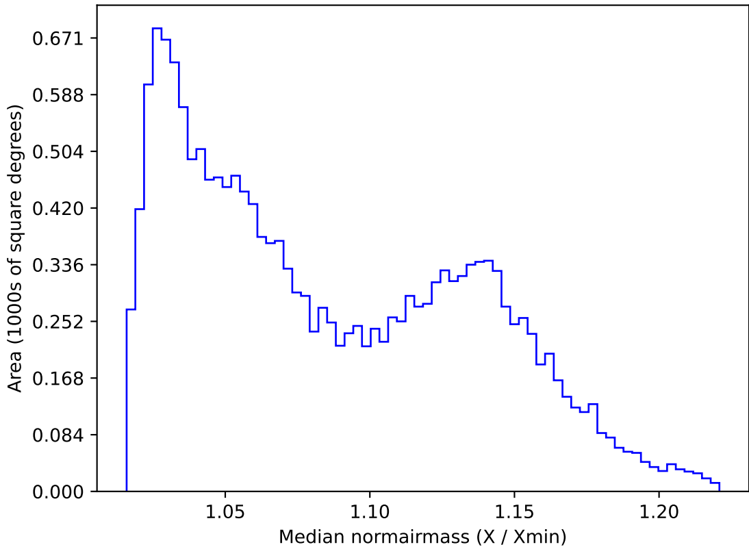
too_elab_r32_d2_griz_v3.4_10yrs WFD g band: Median normairmass
