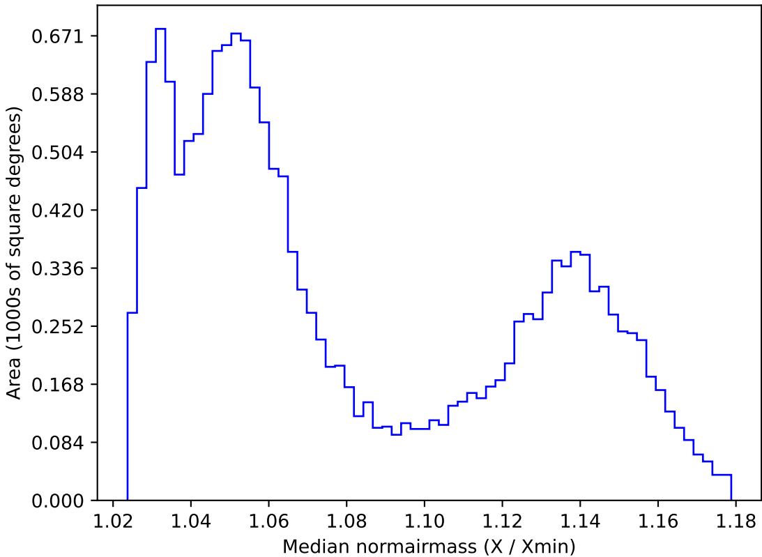
too_elab_r32_d2_griz_v3.4_10yrs WFD all bands: Median normairmass
