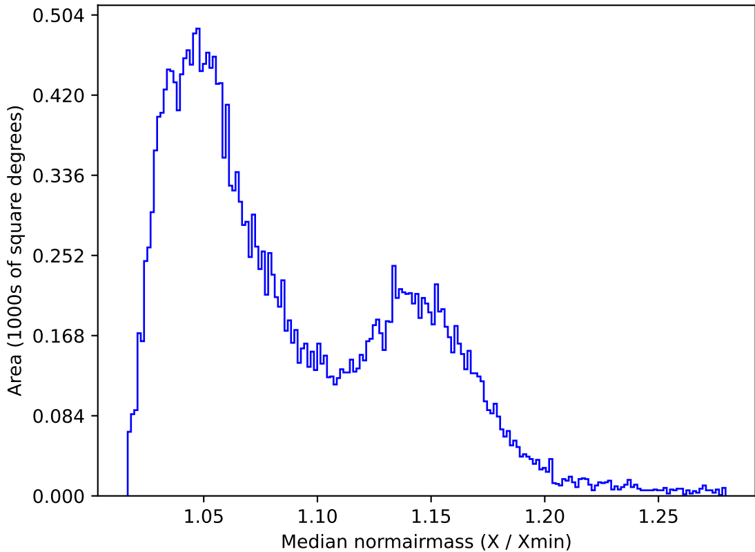
too_elab_r32_d2_griz_v3.4_10yrs All sky z band: Median normairmass
