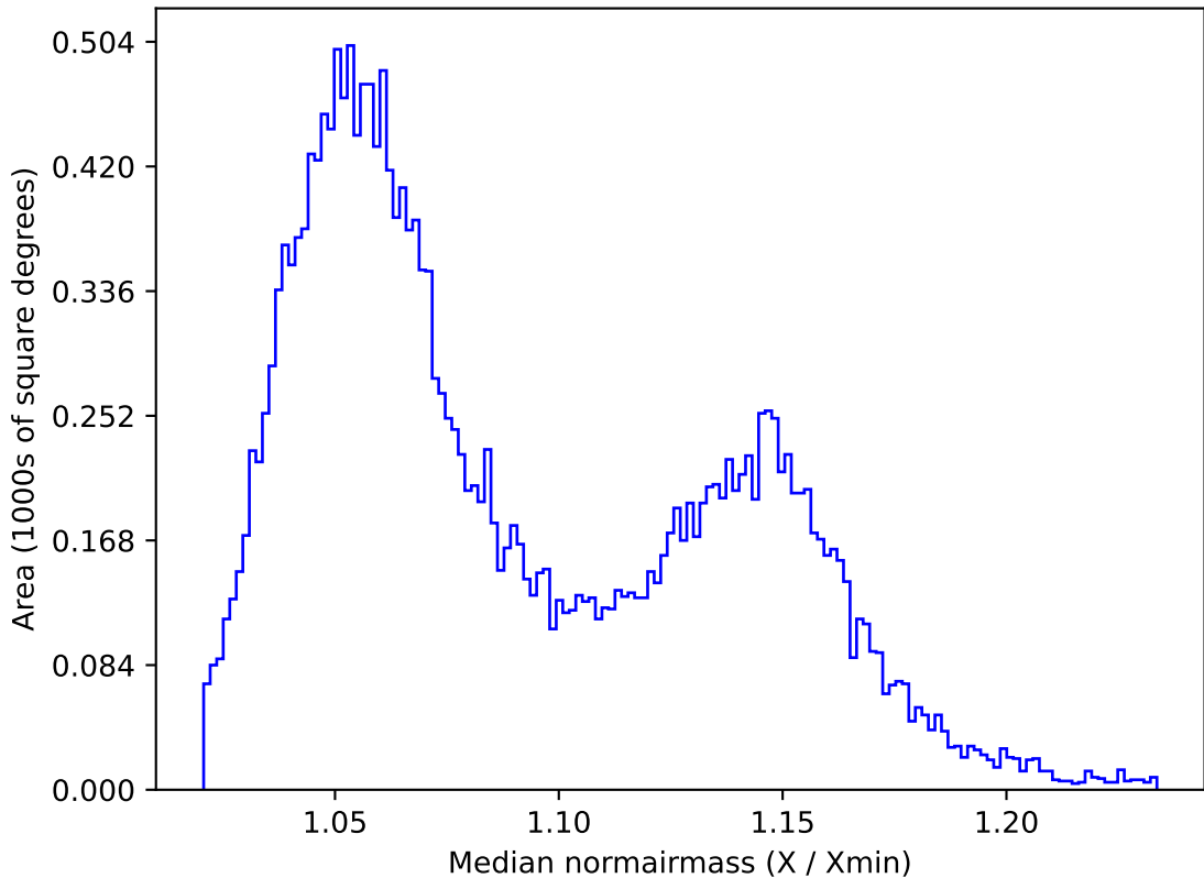
too_elab_r32_d2_griz_v3.4_10yrs All sky y band: Median normairmass
