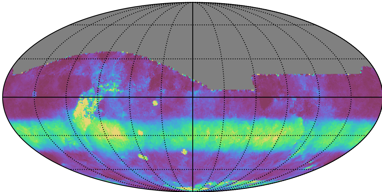
too_elab_r32_d2_griz_v3.4_10yrs All sky r band: Median normairmass
