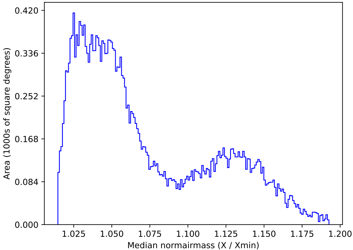
too_elab_r32_d2_griz_v3.4_10yrs All sky r band: Median normairmass
