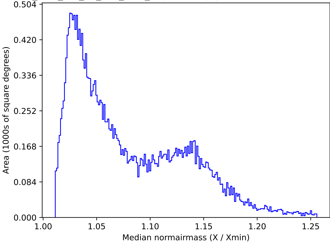
too_elab_r32_d2_griz_v3.4_10yrs All sky g band: Median normairmass
