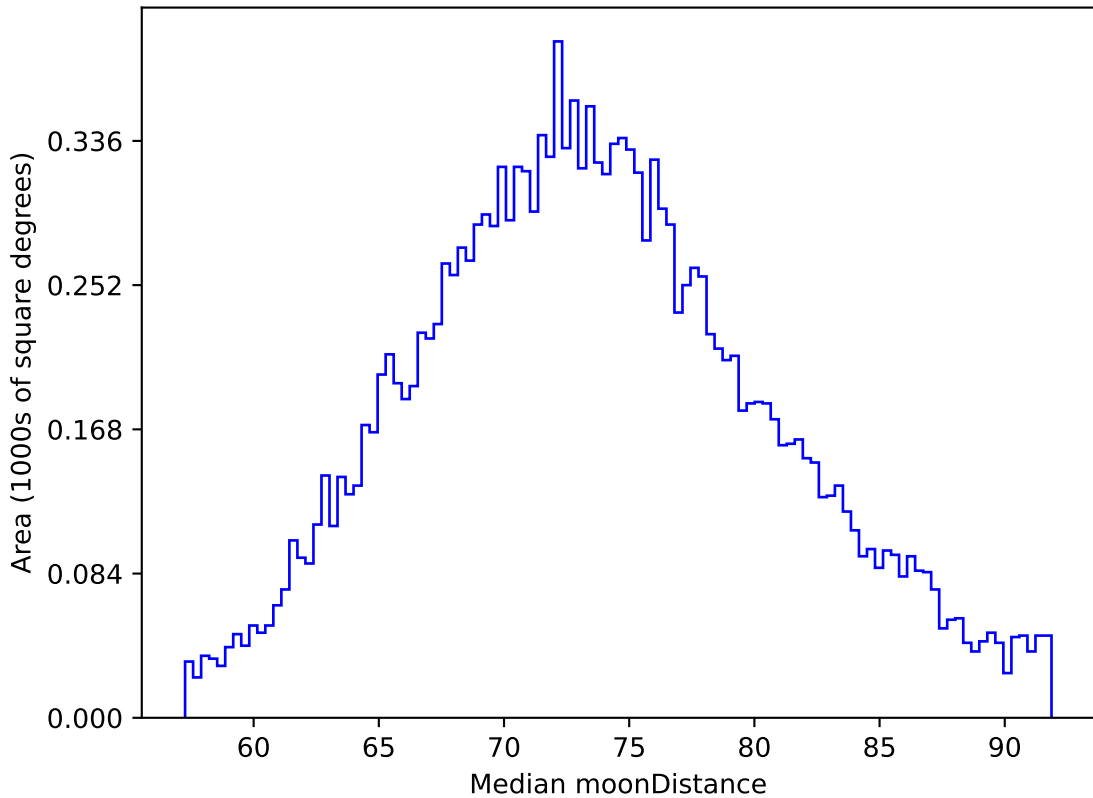
too_elab_r32_d2_griz_v3.4_10yrs WFD z band: Median moonDistance
