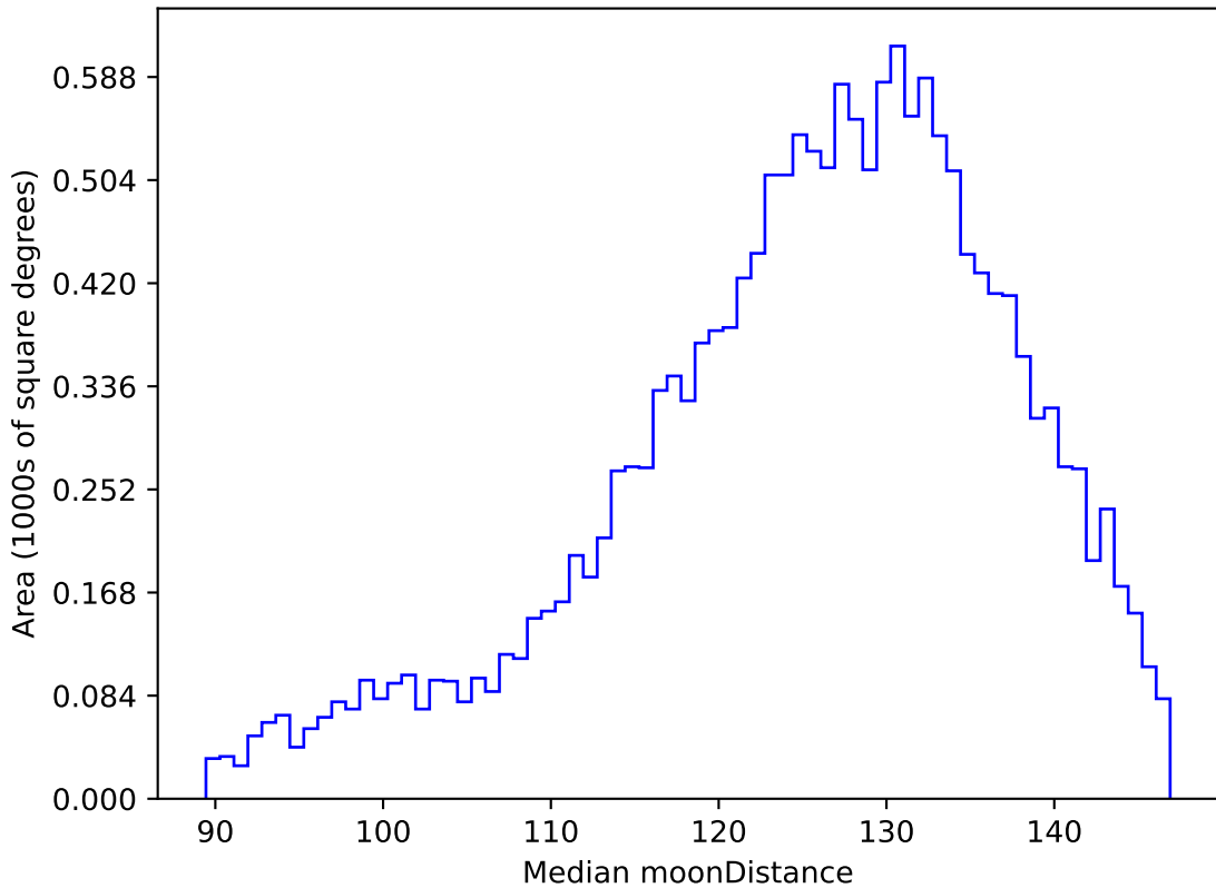
too_elab_r32_d2_griz_v3.4_10yrs WFD u band: Median moonDistance
