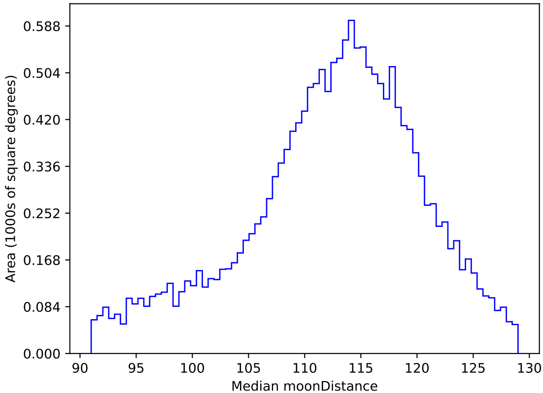
too_elab_r32_d2_griz_v3.4_10yrs WFD r band: Median moonDistance
