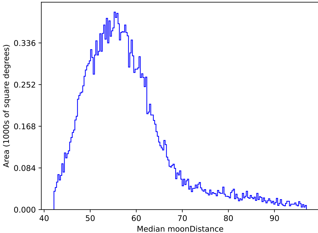
too_elab_r32_d2_griz_v3.4_10yrs All sky y band: Median moonDistance
