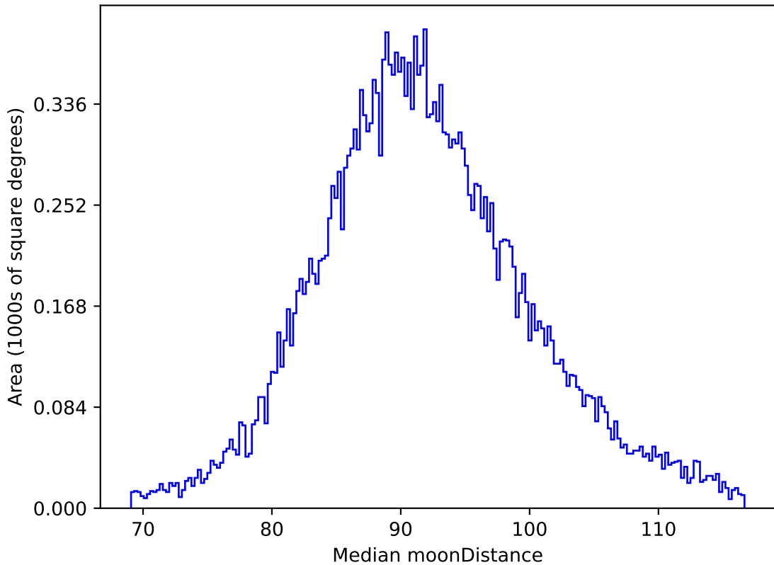
too_elab_r32_d2_griz_v3.4_10yrs All sky i band: Median moonDistance
