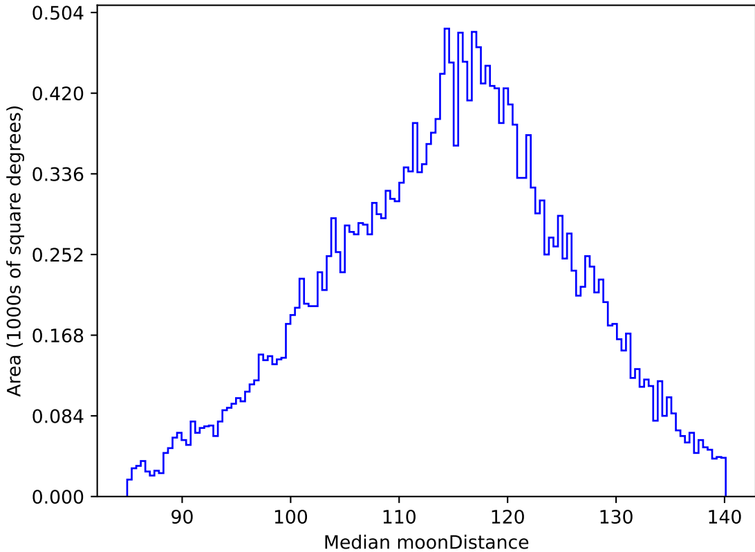
too_elab_r32_d2_griz_v3.4_10yrs All sky g band: Median moonDistance
