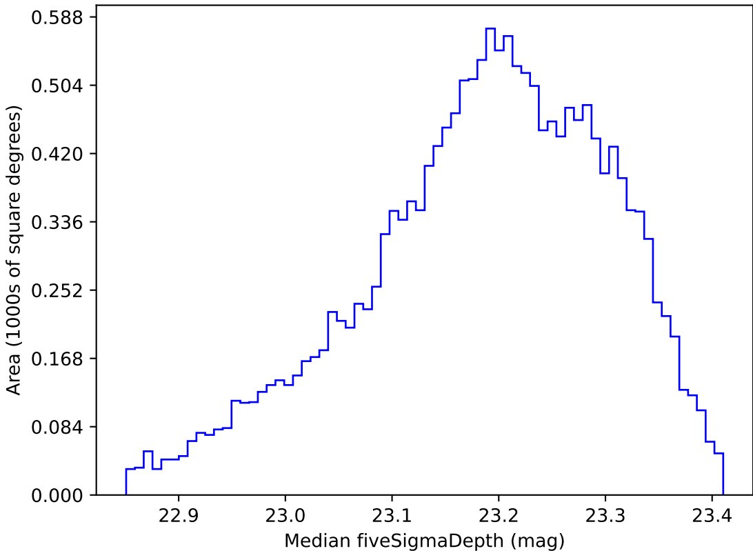
too_elab_r32_d2_griz_v3.4_10yrs WFD u band: Median fiveSigmaDepth
