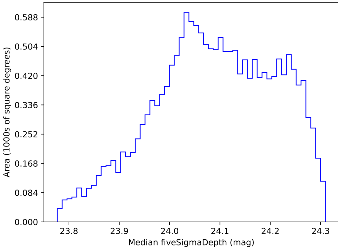
too_elab_r32_d2_griz_v3.4_10yrs WFD r band: Median fiveSigmaDepth
