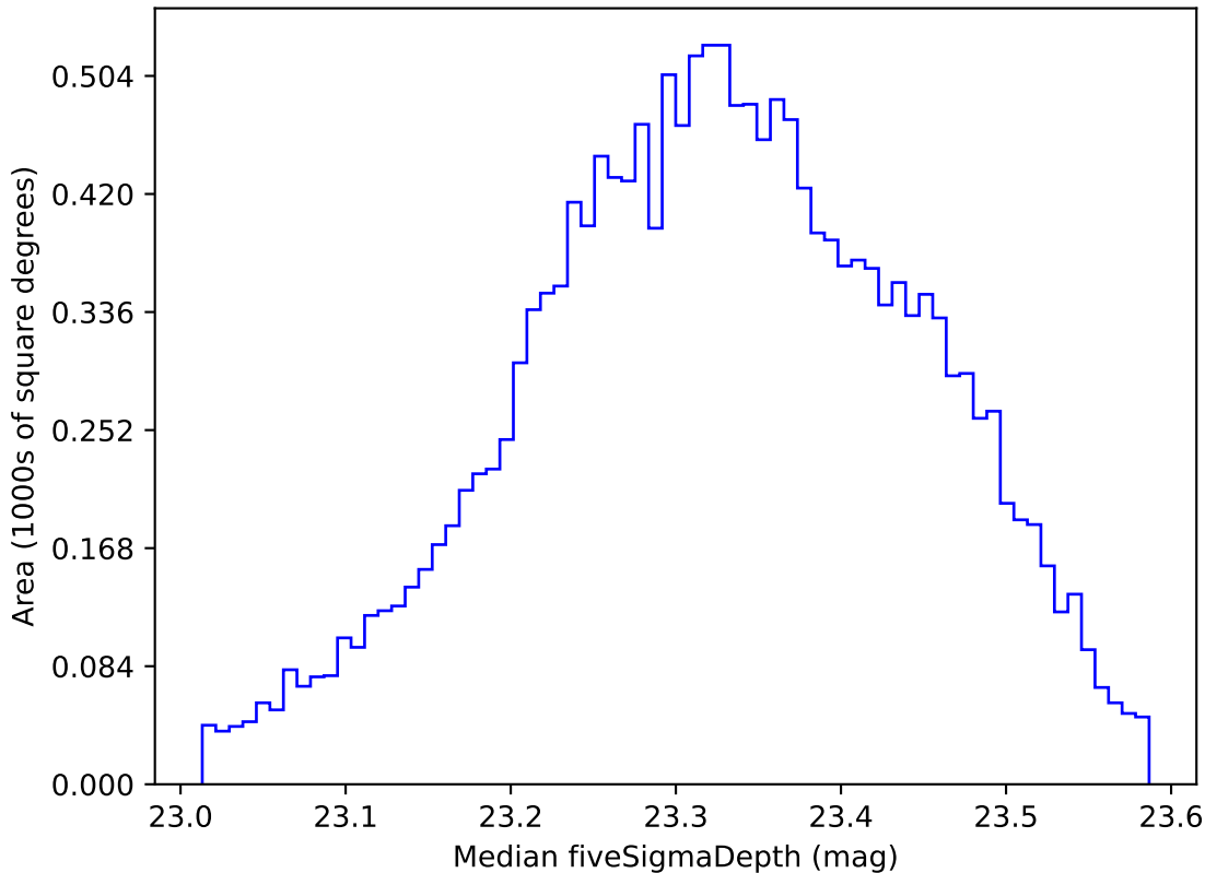
too_elab_r32_d2_griz_v3.4_10yrs WFD all bands: Median fiveSigmaDepth
