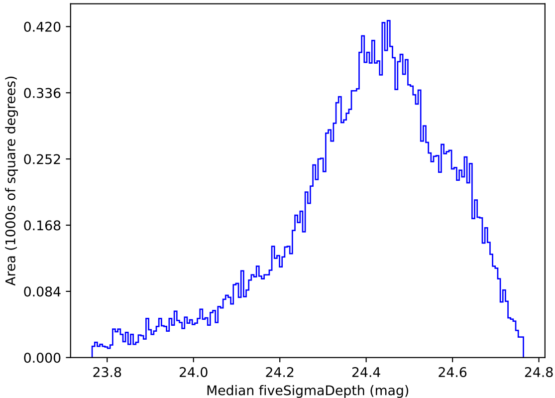
too_elab_r32_d2_griz_v3.4_10yrs All sky g band: Median fiveSigmaDepth
