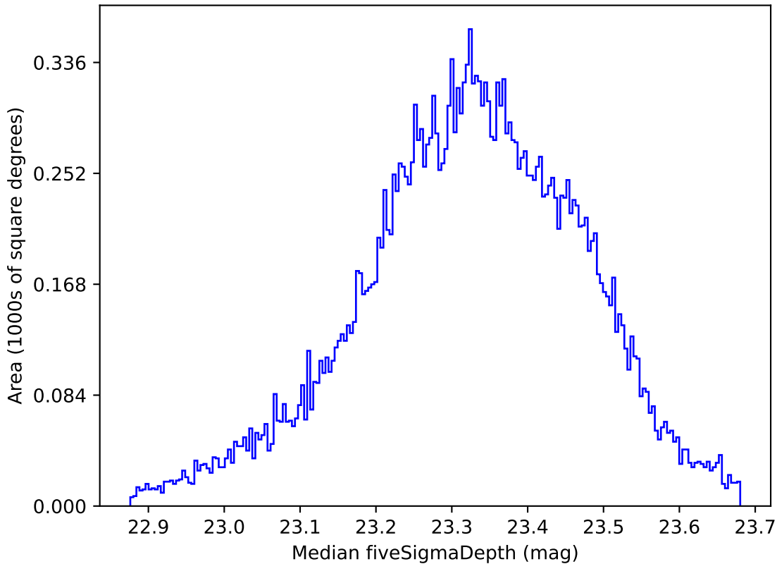
too_elab_r32_d2_griz_v3.4_10yrs All sky all bands: Median fiveSigmaDepth
