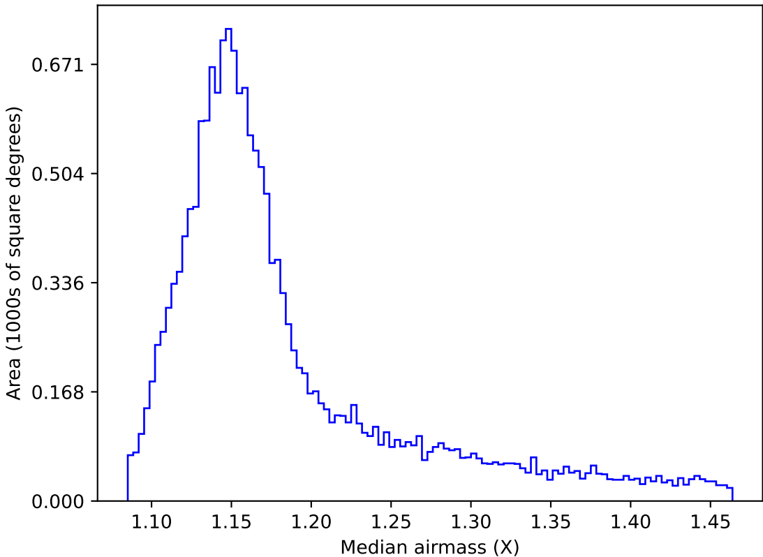
too_elab_r32_d2_griz_v3.4_10yrs WFD z band: Median airmass
