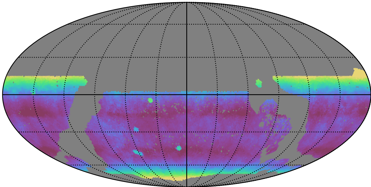
too_elab_r32_d2_griz_v3.4_10yrs WFD y band: Median airmass
