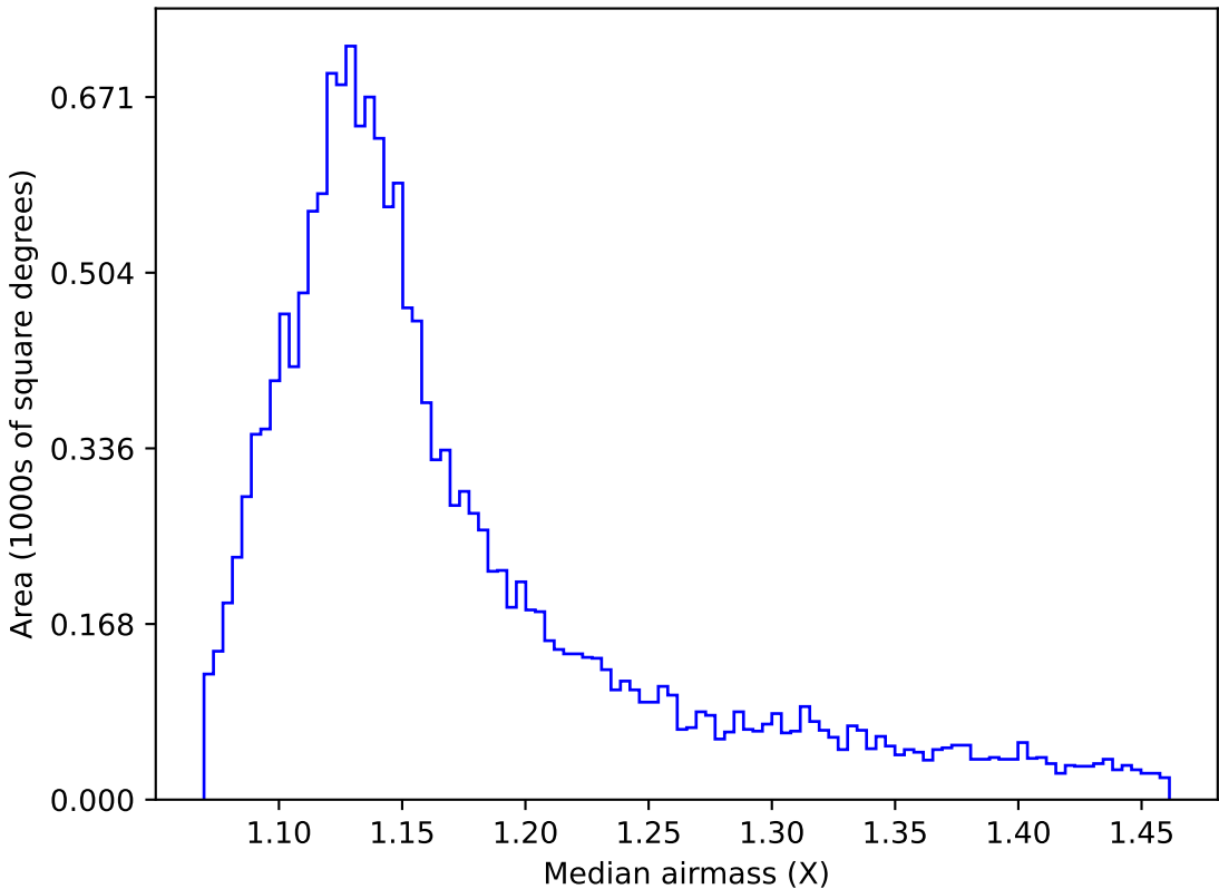
too_elab_r32_d2_griz_v3.4_10yrs WFD u band: Median airmass
