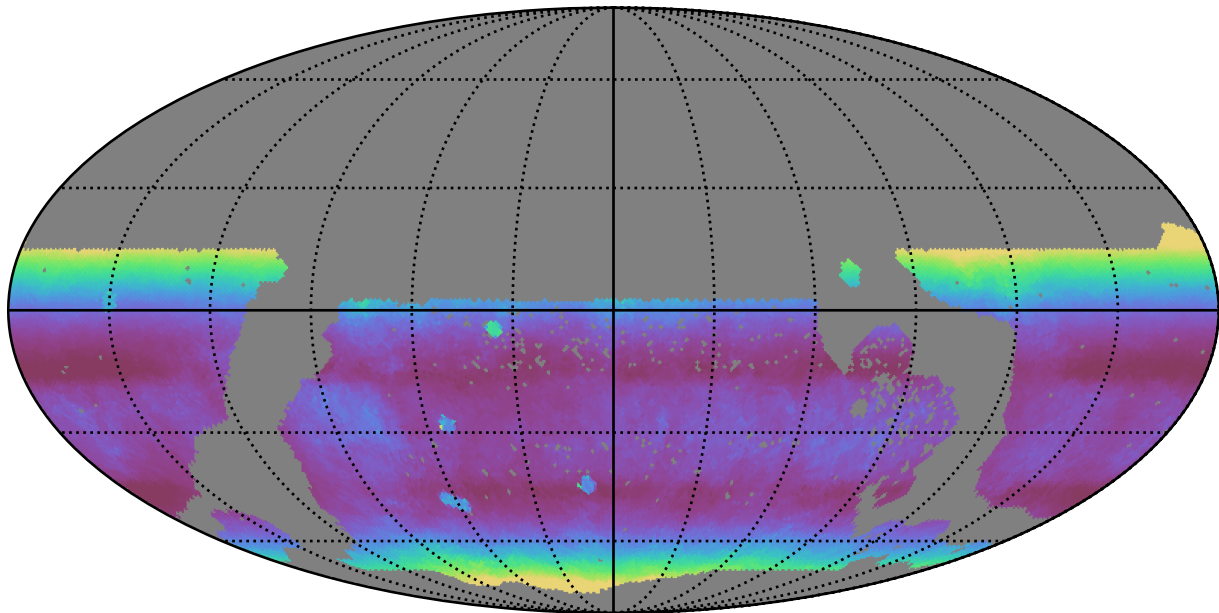
too_elab_r32_d2_griz_v3.4_10yrs WFD r band: Median airmass
