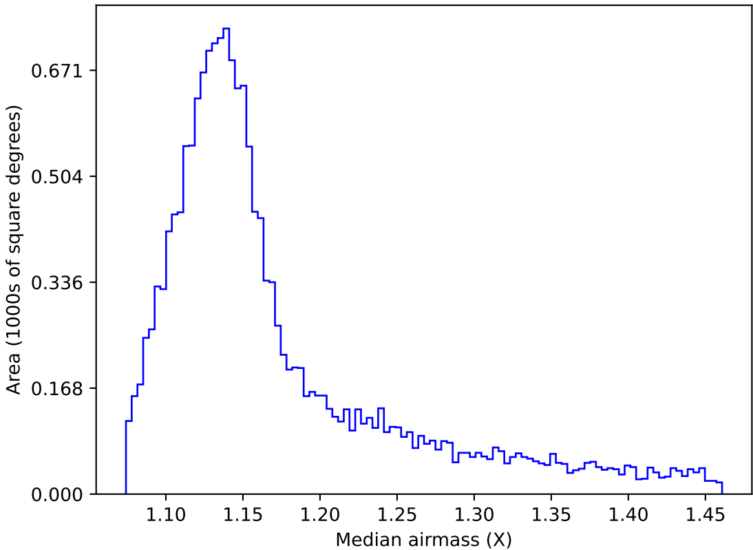
too_elab_r32_d2_griz_v3.4_10yrs WFD r band: Median airmass
