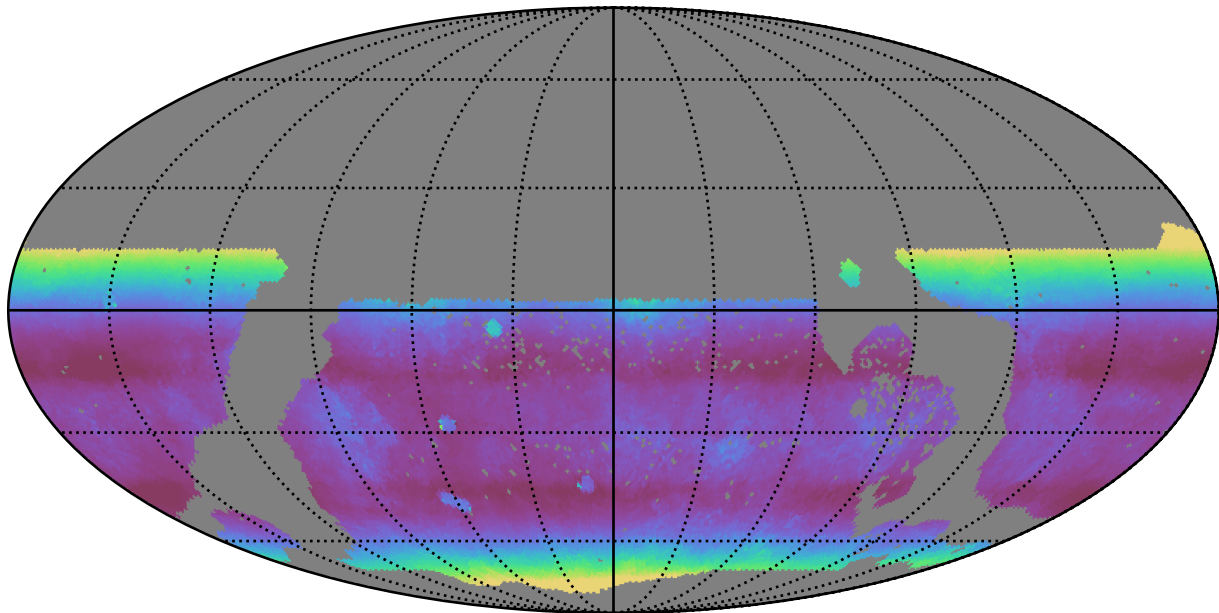
too_elab_r32_d2_griz_v3.4_10yrs WFD i band: Median airmass
