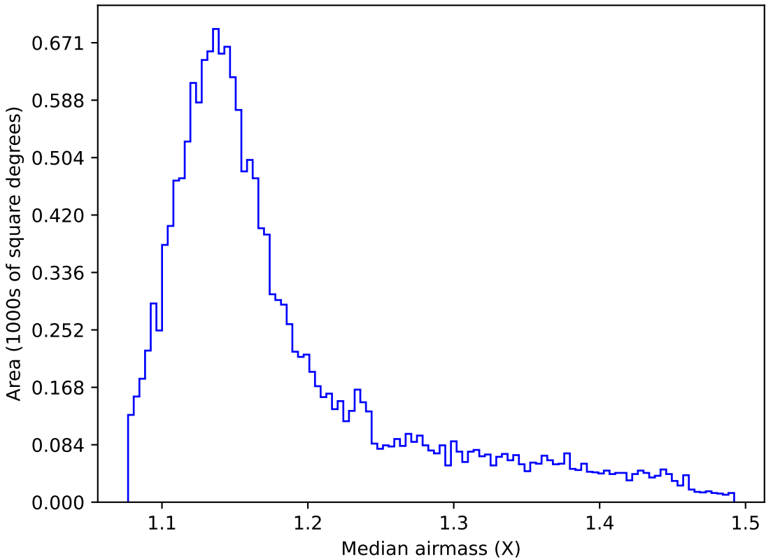
too_elab_r32_d2_griz_v3.4_10yrs WFD g band: Median airmass
