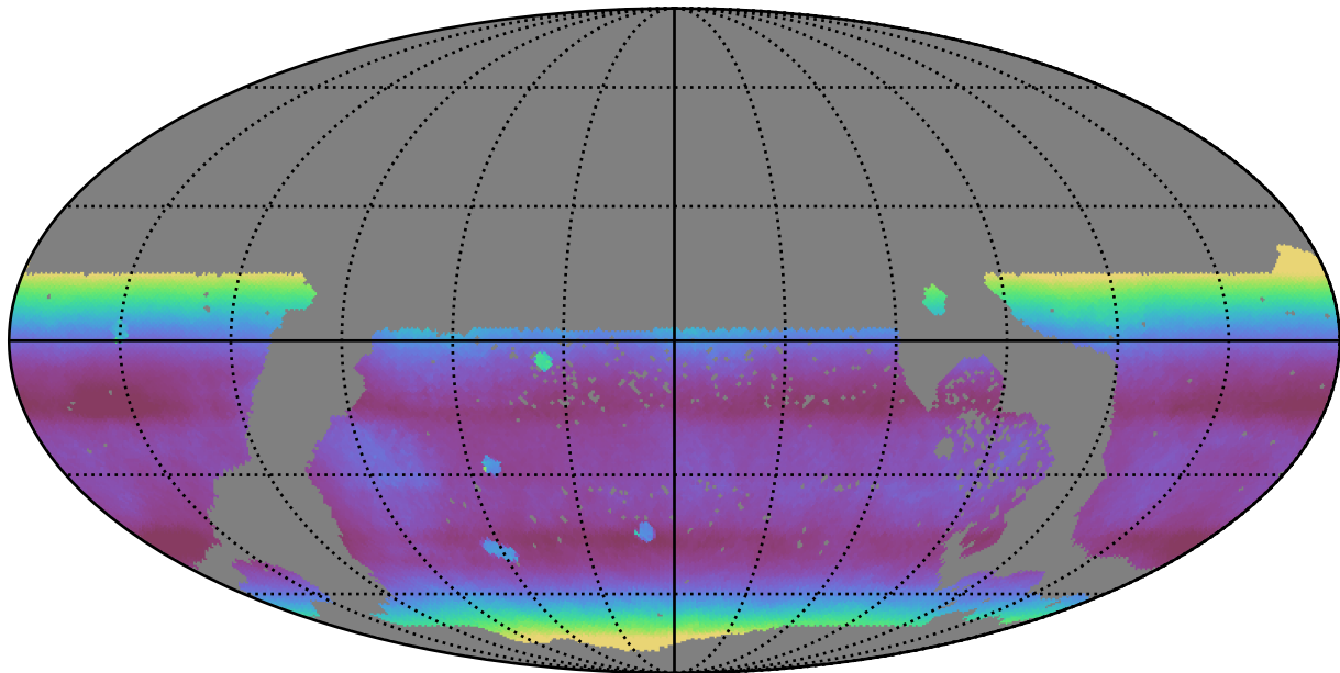
too_elab_r32_d2_griz_v3.4_10yrs WFD all bands: Median airmass
