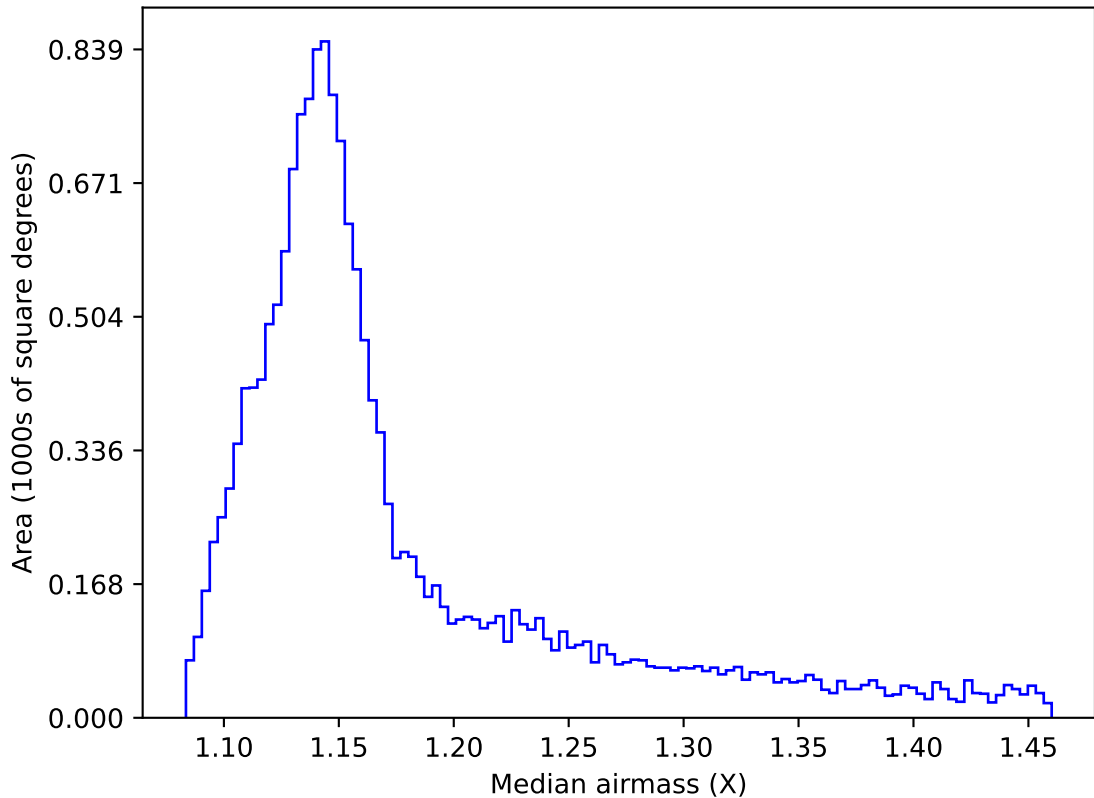
too_elab_r32_d2_griz_v3.4_10yrs WFD all bands: Median airmass
