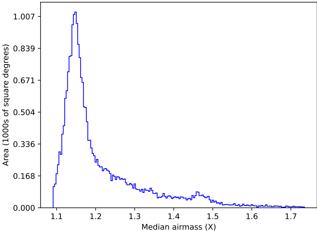
too_elab_r32_d2_griz_v3.4_10yrs All sky y band: Median airmass
