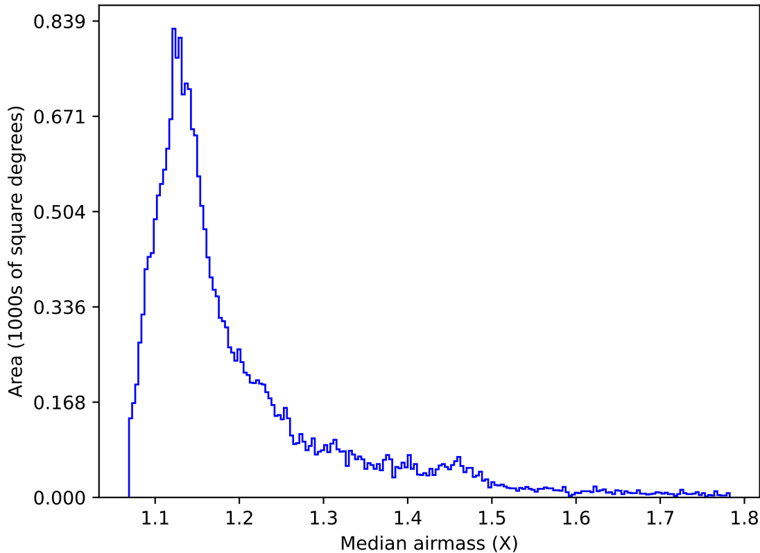
too_elab_r32_d2_griz_v3.4_10yrs All sky u band: Median airmass
