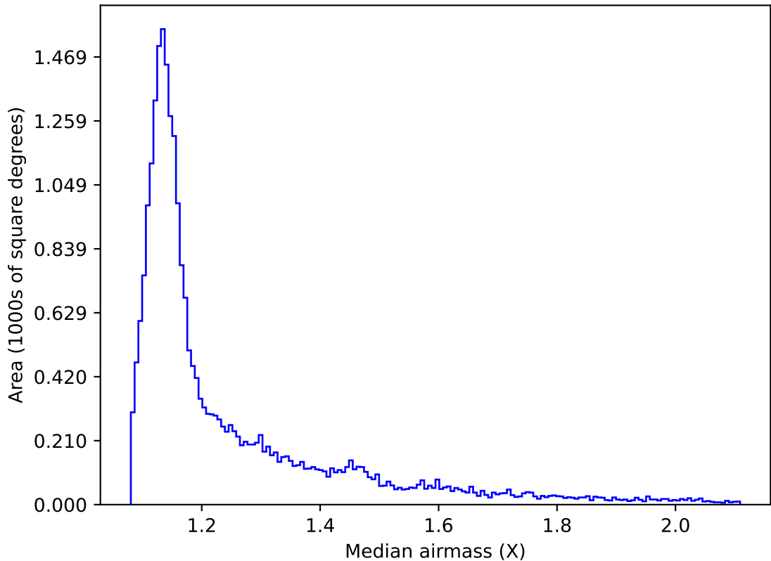
too_elab_r32_d2_griz_v3.4_10yrs All sky i band: Median airmass
