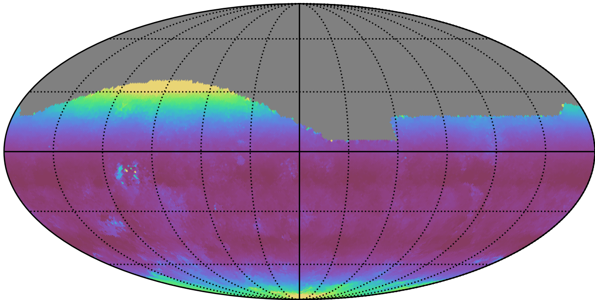
too_elab_r32_d2_griz_v3.4_10yrs All sky g band: Median airmass
