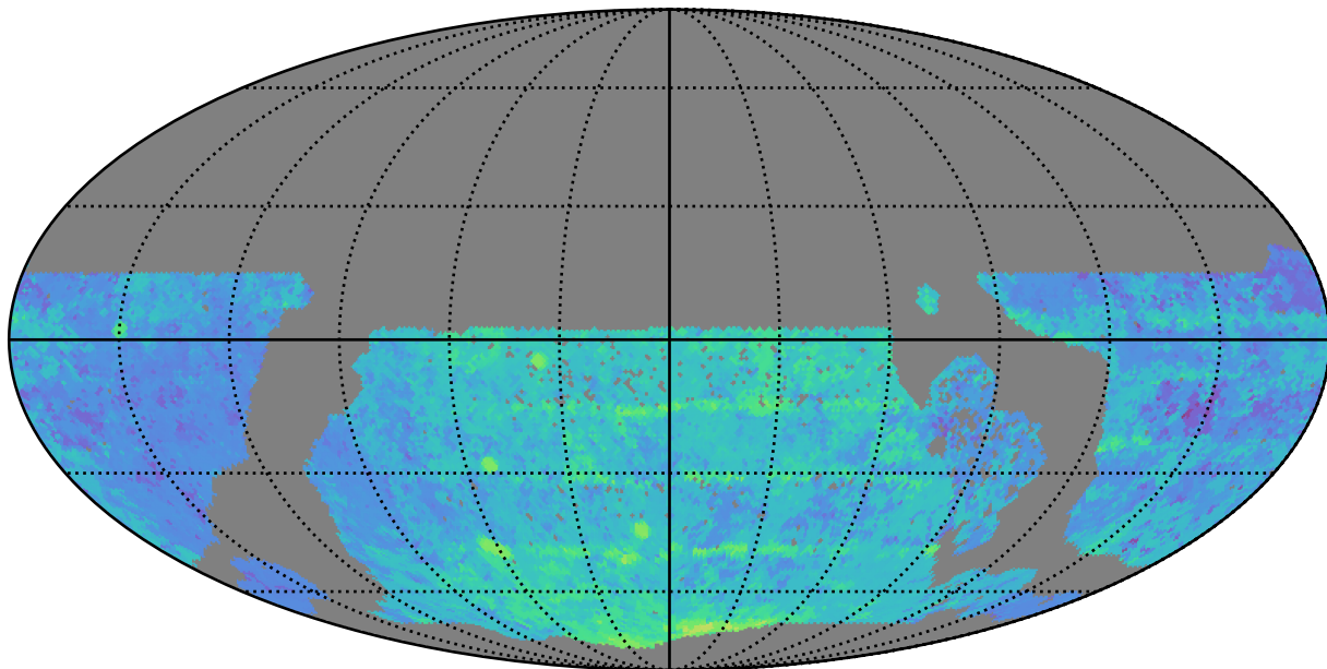
too_elab_r32_d2_griz_v3.4_10yrs WFD y band: Median Season Length
