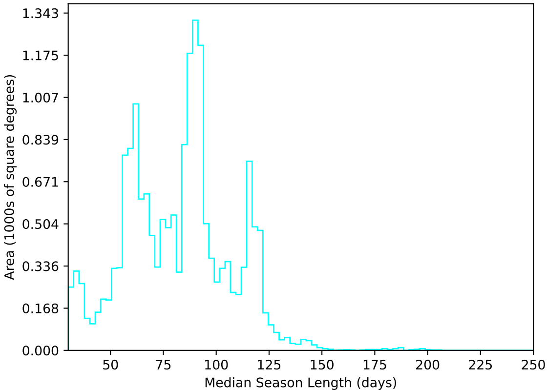
too_elab_r32_d2_griz_v3.4_10yrs WFD u band: Median Season Length
