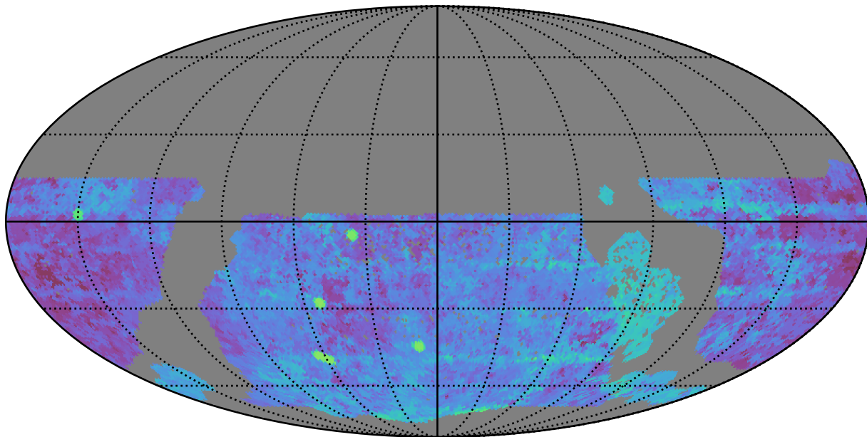
too_elab_r32_d2_griz_v3.4_10yrs WFD g band: Median Season Length
