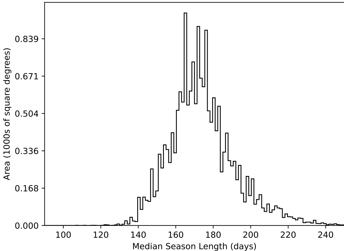
too_elab_r32_d2_griz_v3.4_10yrs WFD all bands: Median Season Length
