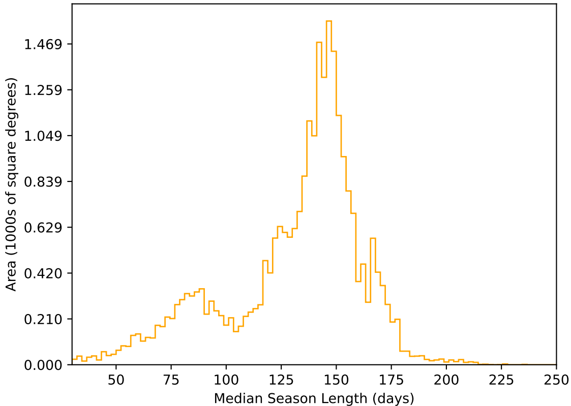
too_elab_r32_d2_griz_v3.4_10yrs All sky r band: Median Season Length
