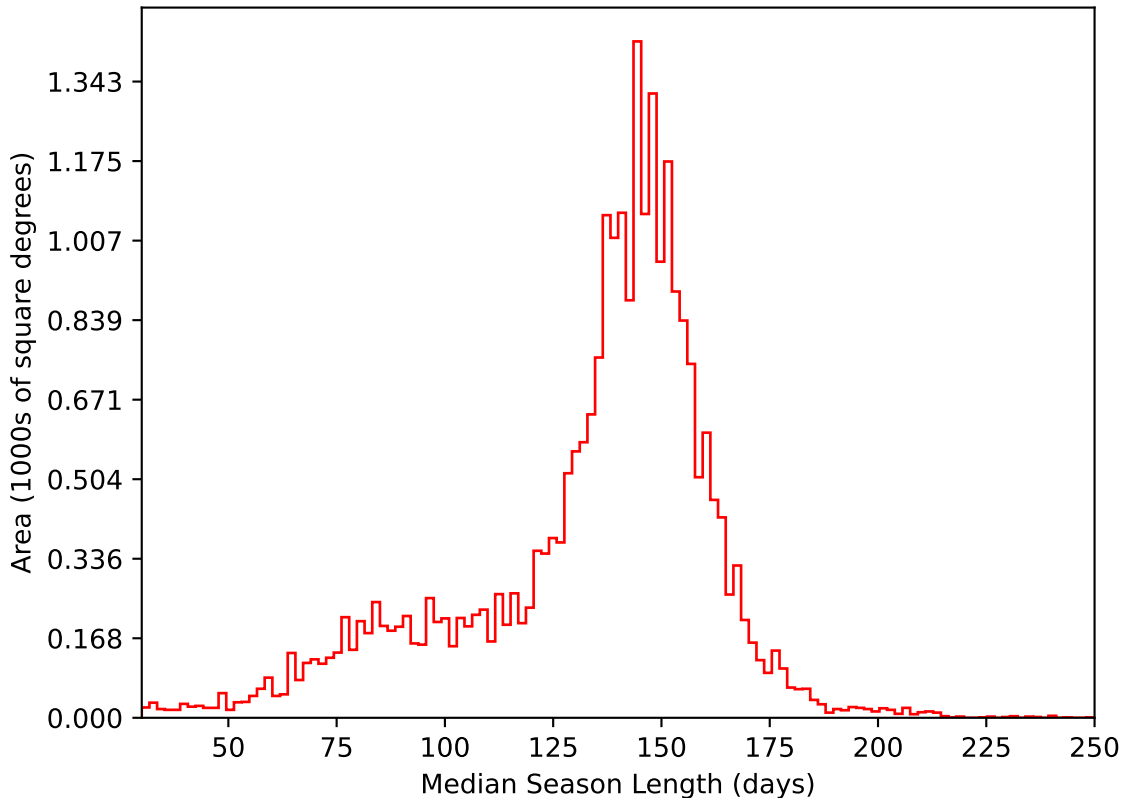
too_elab_r32_d2_griz_v3.4_10yrs All sky i band: Median Season Length
