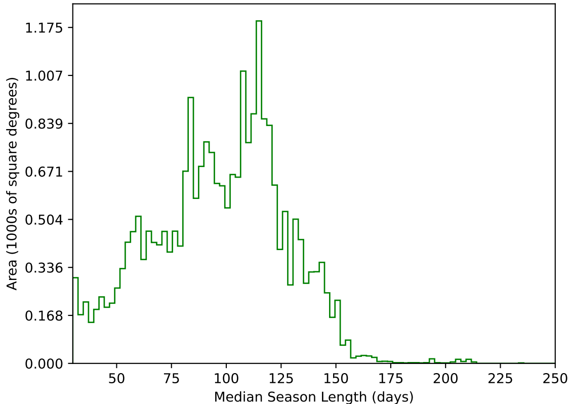
too_elab_r32_d2_griz_v3.4_10yrs All sky g band: Median Season Length
