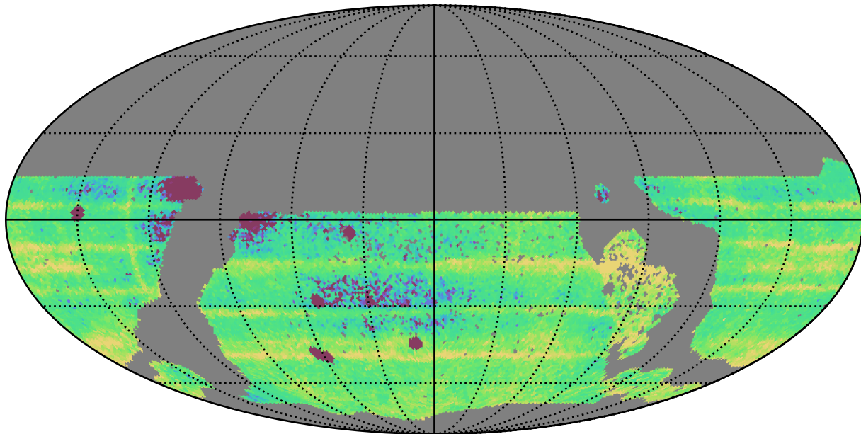
too_elab_r32_d2_griz_v3.4_10yrs WFD: Median Intra-Night Gap
